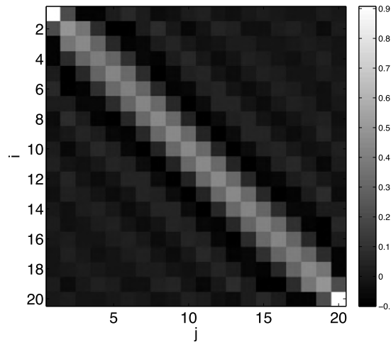
Figure 4.8 Resolution matrix for the Shaw problem, \alpha = 4.29 \times 10^{-5} . Note that the noise-free inversion of a spike model e_j will produce the j th column or row of \mathbf{R}_m (e.g., Fig. 4.7 is a plot of the 10th column/row).
