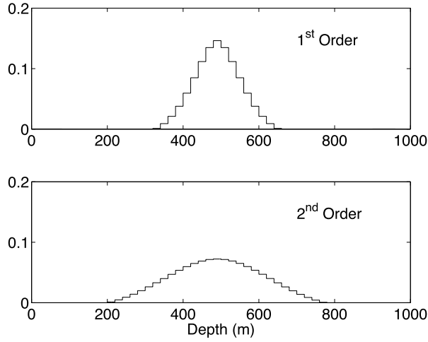
Figure 4.17 The model resolution matrix \mathbf{R}_{\alpha,L} multiplied times the spike model for the first- and second-order regularized solutions of Example 4.4.
