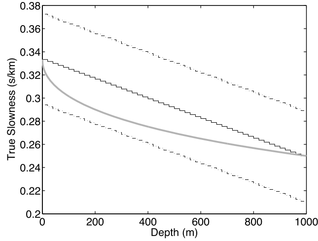
Figure 11.9 A constant-slowness gradient prior distribution and its 95% distribution intervals for the VSP problem. The true model is shown as the gray smooth curve.
