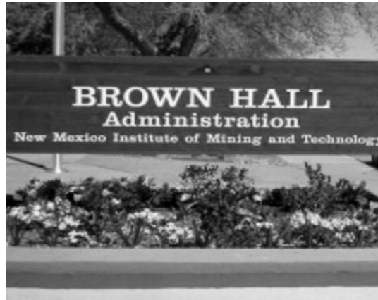
Figure 7.10 An image before discrete cosine transform threshholding.
