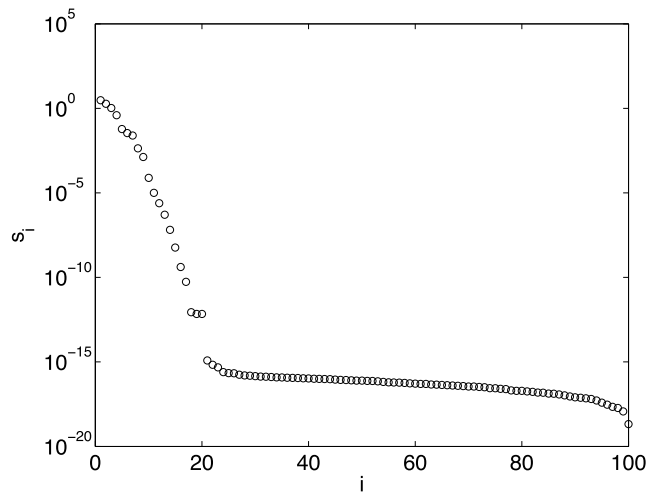
Figure 3.26 Singular values of \mathbf{G} for the Shaw example ( n = m = 100 ).
