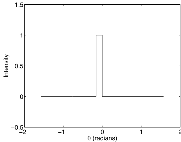
Figure 3.21 The spike model.
