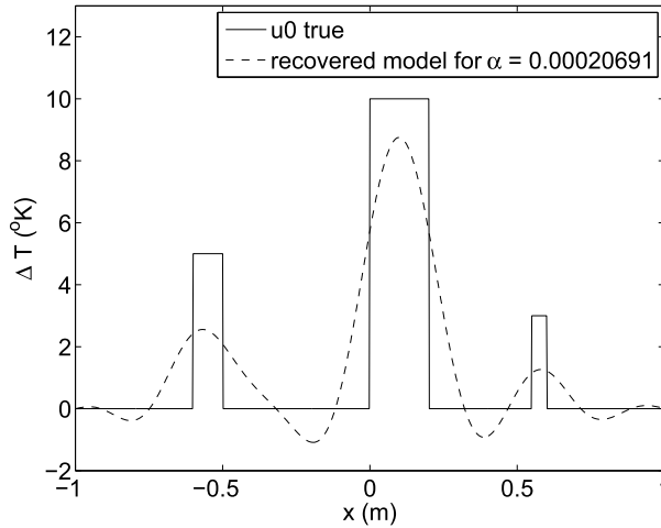
Figure 10.13 True initial condition and inverse solution with regularization parameter determined from the discrepancy principle as shown in Fig. 10.12.
