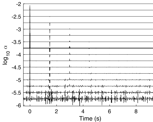
Figure 7.8 1-norm regularized solutions corresponding to the L-curve shown in Fig. 7.7. Model corresponding to the L-curve corner is shown in bold and is reproduced in Fig. 7.9.
