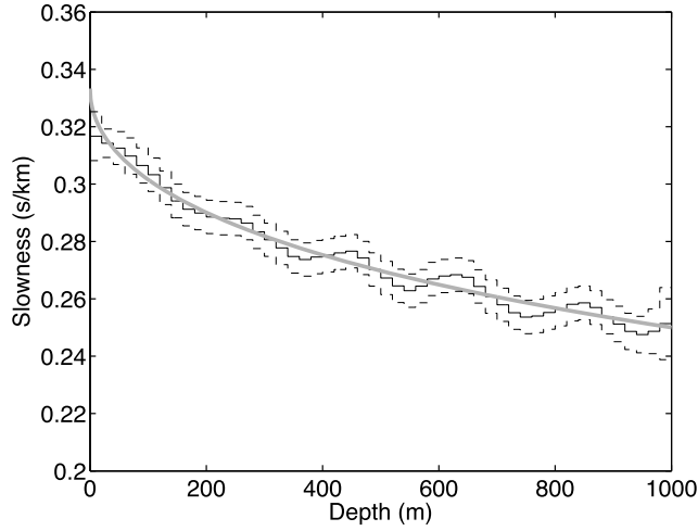
Figure 11.11 MAP model obtained from the posterior distribution, and its 95% distribution intervals, using the prior distribution described in Figs. 11.9 and 11.10. The true model is shown as the gray smooth curve.
